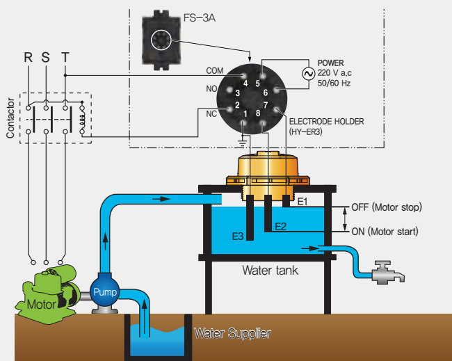
Example of Water Supply connection (FS-3A)
