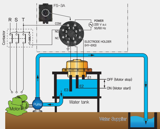
Example of Drain connection (FS-3A)
